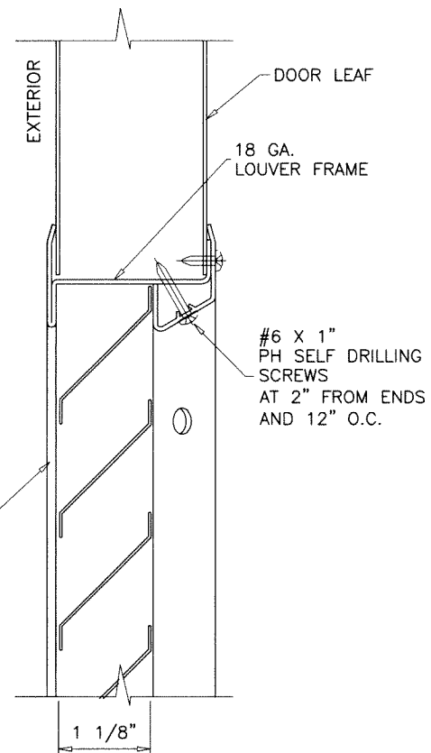
LOUVER DETAIL (OPTION 2)
