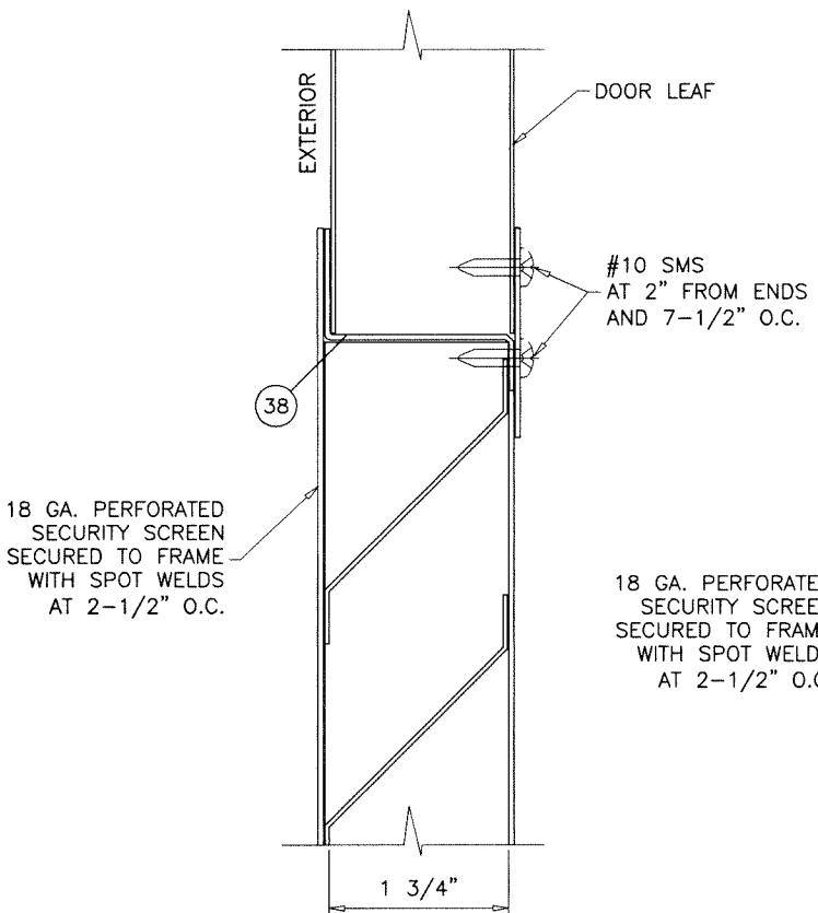
LOUVER DETAIL (OPTION 1)
