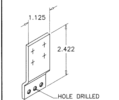
10 REINF. PLATE
