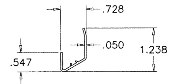
43B LOUVER FRAME INTERIOR (1")
