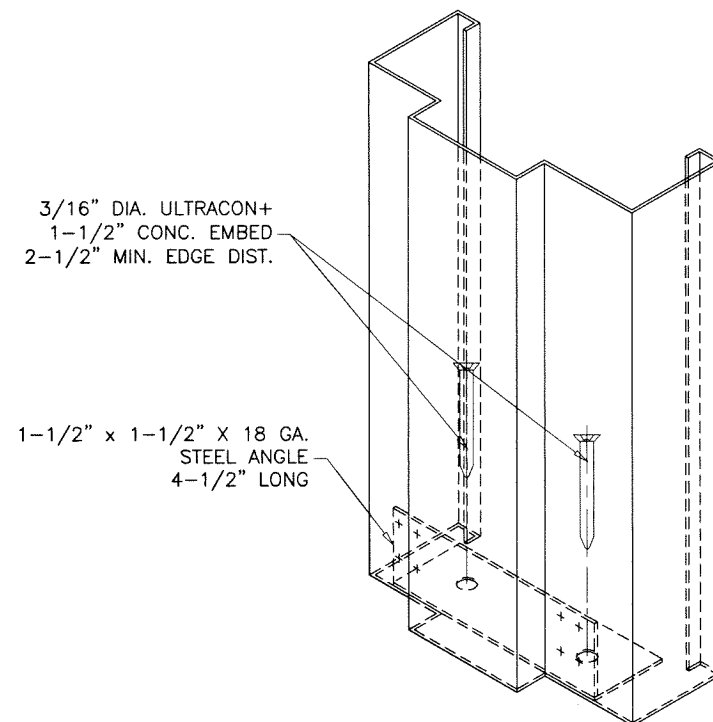
BOTTOM CORNER ANCHOR DETAIL OPTIONAL
