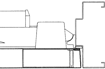
LOCK STILE SINGLE DOOR
