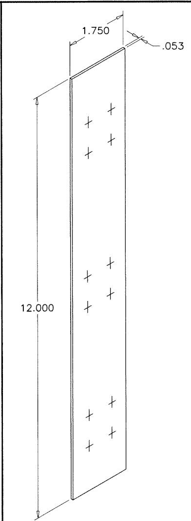
10 REINF. PLATE
