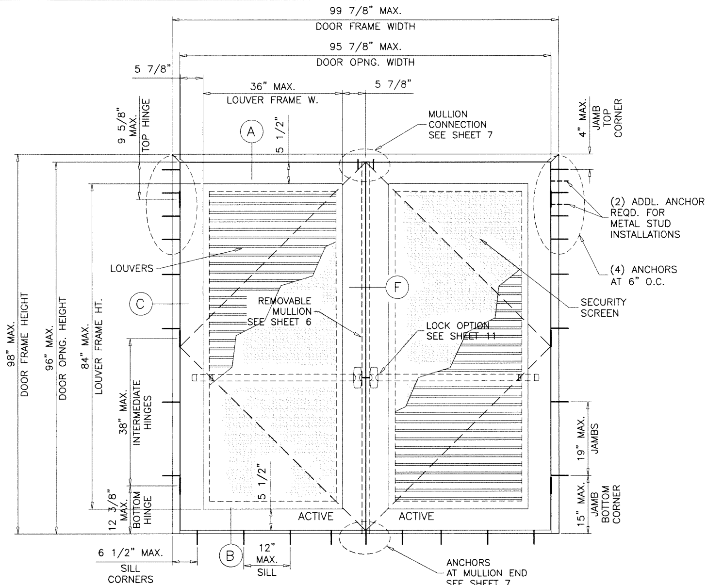
TYPICAL ELEVATION ( X-X WITH MULLION)
